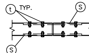
INTERNAL SPLICE DETAIL (8 PLACES)
