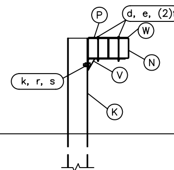
LINE POSTS With Extended Block (P) POSTS 9-12, 16-19, 23-26 (24 PLACES TOTAL)
