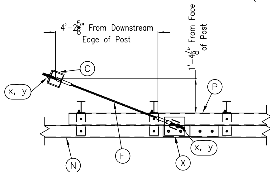
BENT SPLICE DETAIL (2 PLACES)
