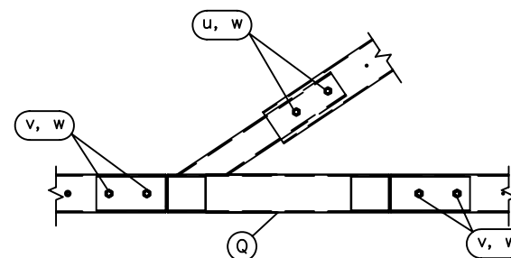
"Y" CONNECTION DETAIL (2 PLACES)
