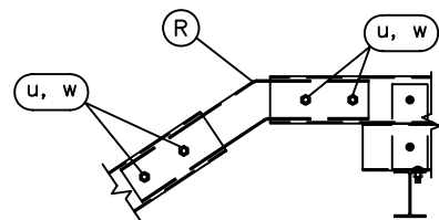
BENT SPLICE DETAIL (2 PLACES)
